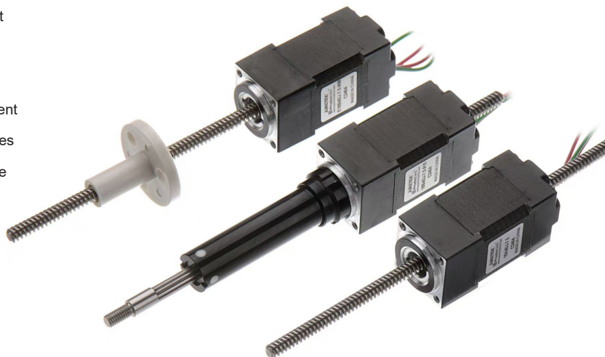
Size 6: 16mm (.6 in) Hybrid Linear Actuator (3° Step Angle)
