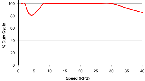
HT34-486 Max Duty Cycle vs Speed 60VDC, 8A parallel 40 °C Ambient on a 10 x 10 x .5 Aluminum Plate
