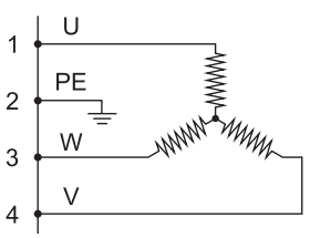
Connector Power Q View: Motor connector, plug side
