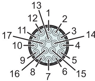
Connector Encoder J View: Motor connector, plug side
