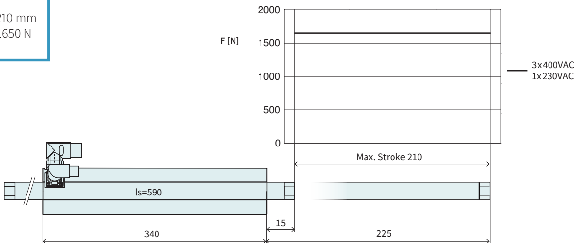
Technical Data P10-70x240U/210
