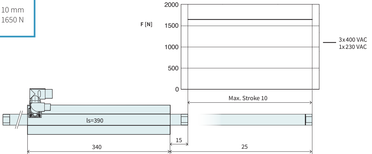
Technical Data P10-70x240U/10
