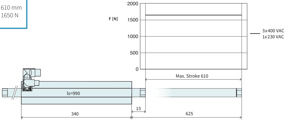
Technical Data P10-70x240U/610
