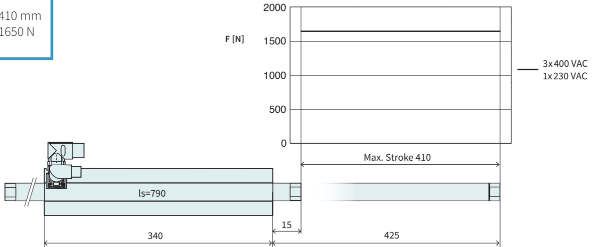
Technical Data P10-70x240U/410
