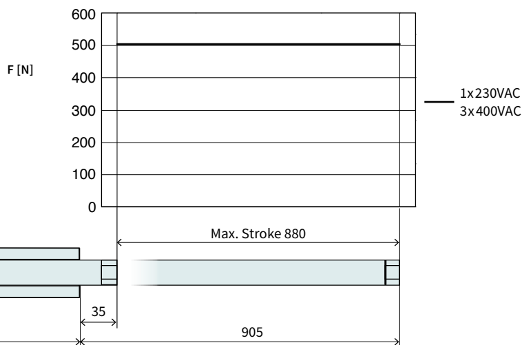
Technical Data P10-54x180U/880
