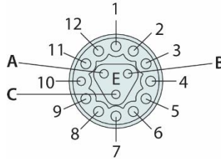
View: Motor connector, plug side
