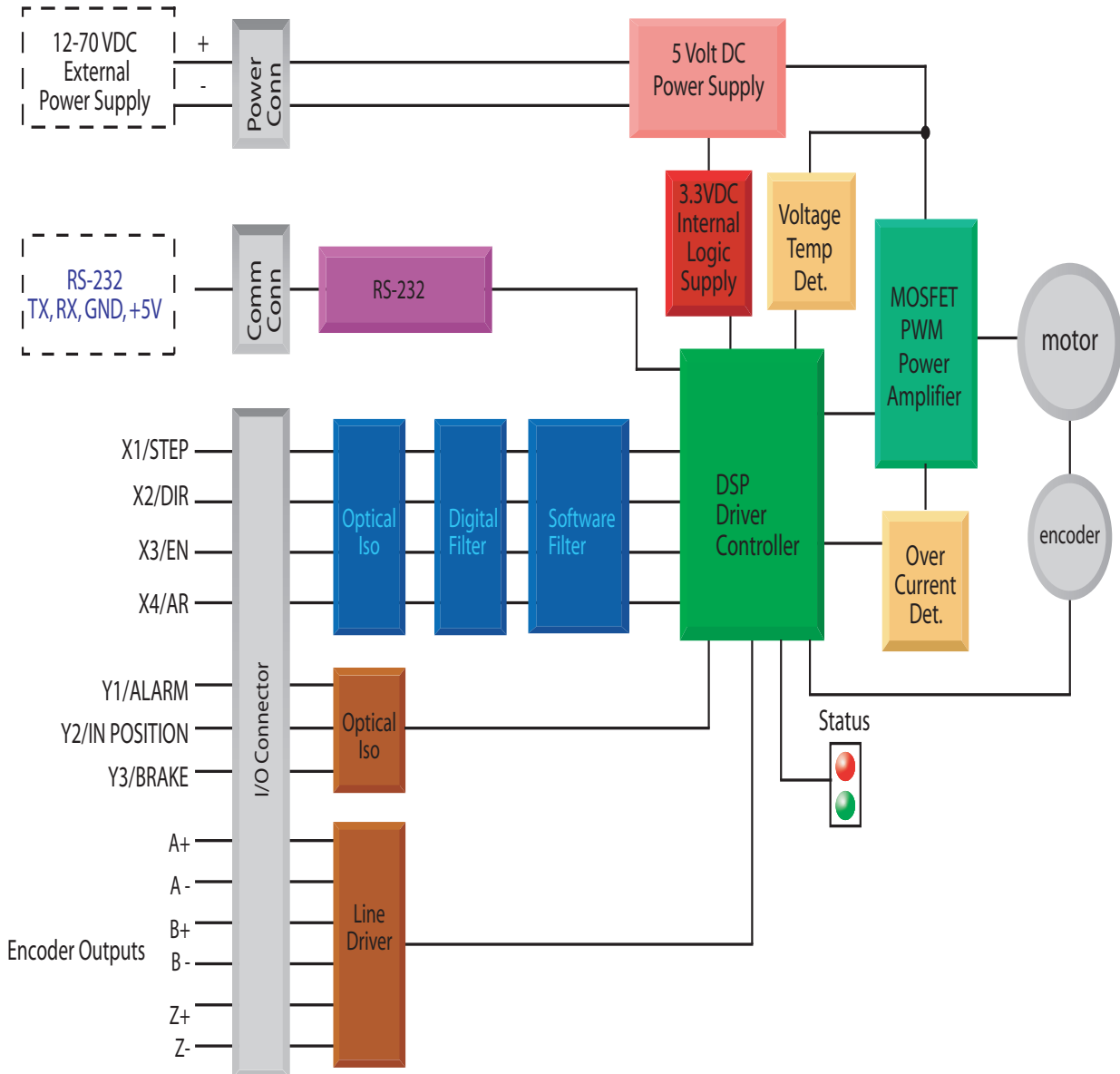
TSM23P Block Diagram
