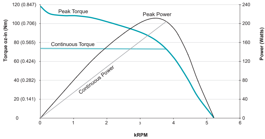
SM23165DT at 42 VDC at rise to 85°C
