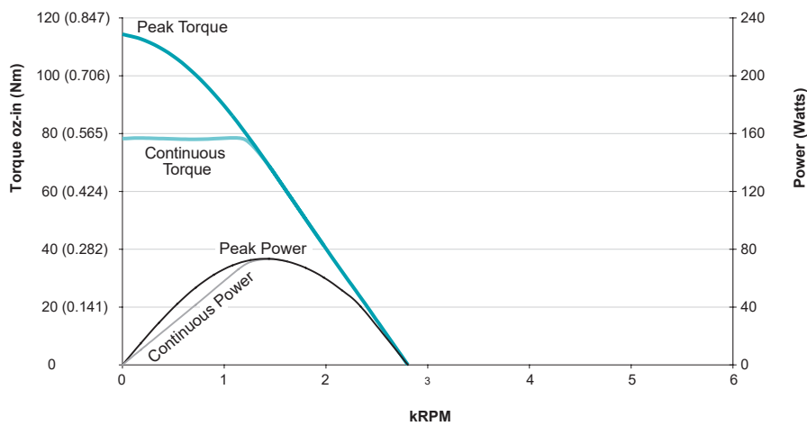
SM23165DT at 24 VDC at rise to 85°C
